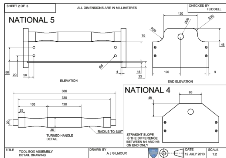
Orthographic Drawing
